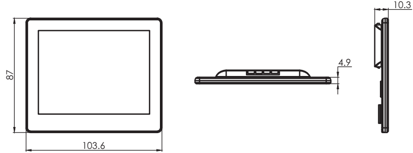
TECHNICAL DRAWINGS (mm)
